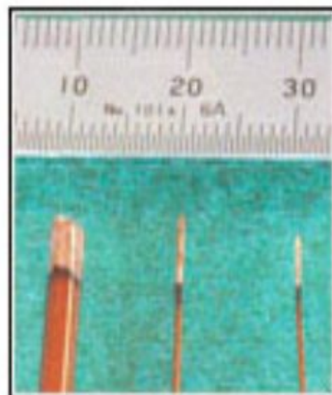
▲ Removal of enamel coating
